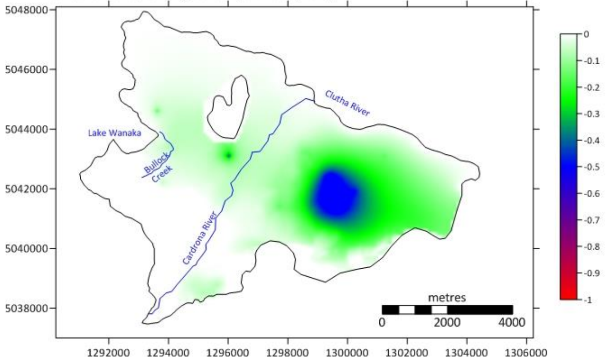
Water level drawdown due to pumping at existing metered rates compared to no pumping scenario (at January 2017)
