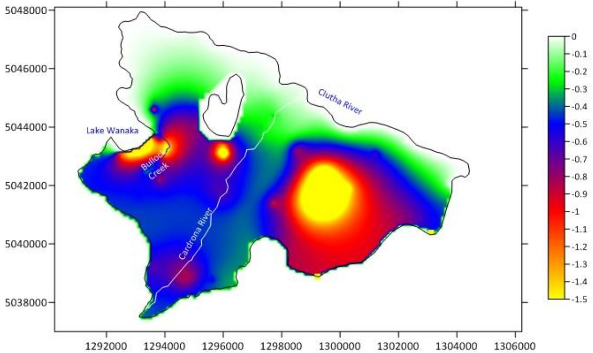
Water level drawdown due to pumping at increased rates ( 5 \times 10^6 \text{ m}^3/\text{year} ) metered rates compared to no pumping scenario (at January 2017)
