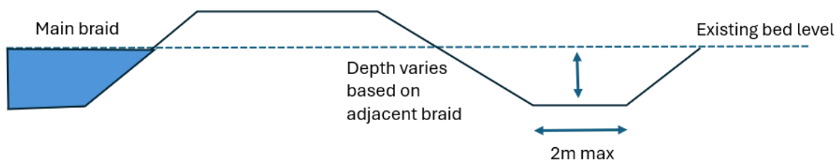
Figure 4: Example cross-section of diversion channel
