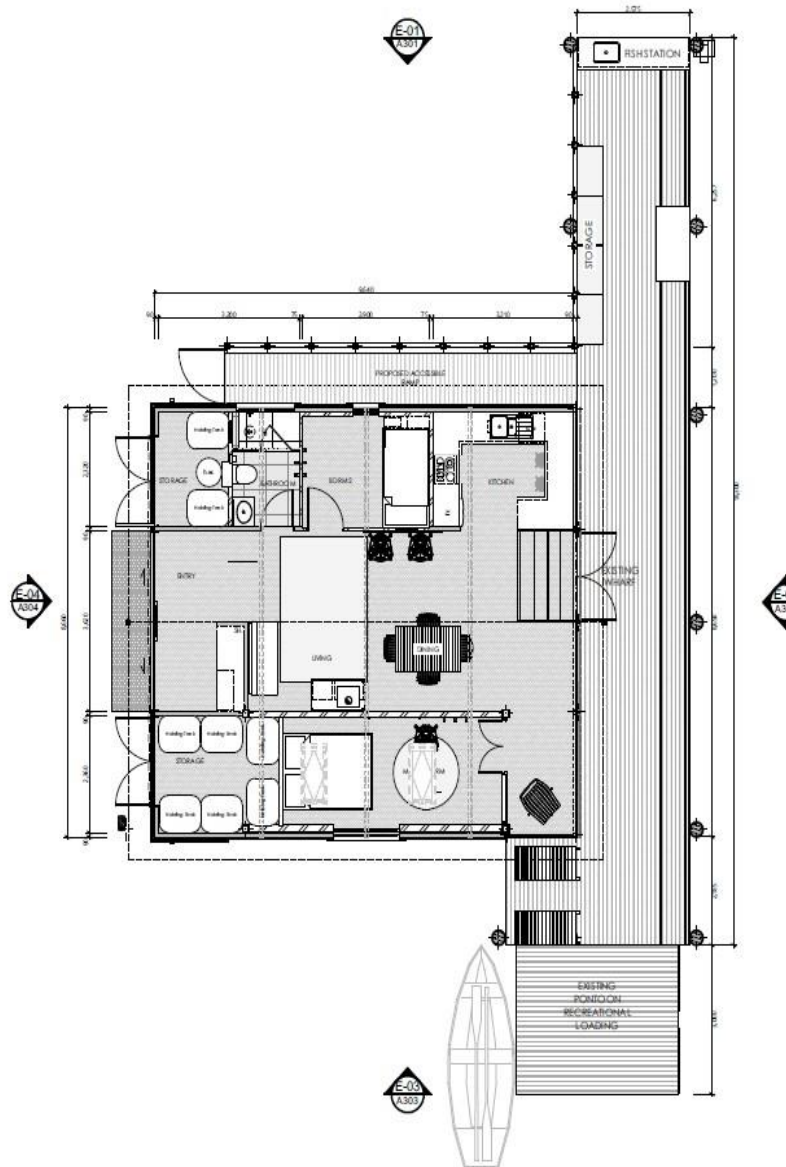
Proposed Ground Floor Plan 1:100
