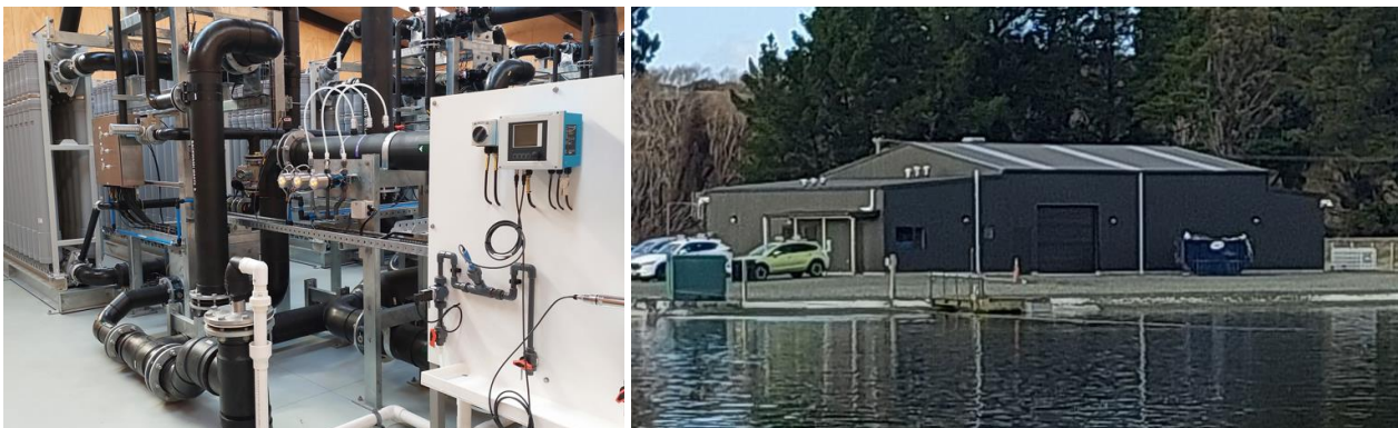
Figure 18 Membrane filtration example installation (Te Anau WWTP)
