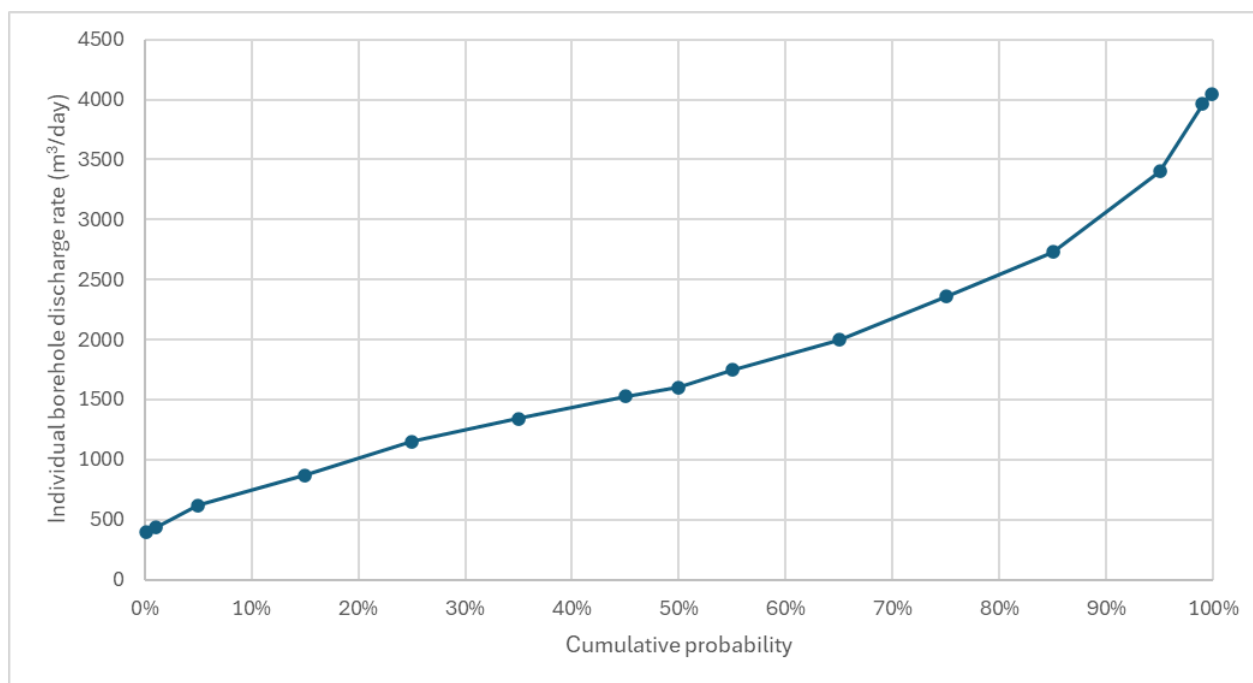
Figure E-2 Individual borehole discharge rate
