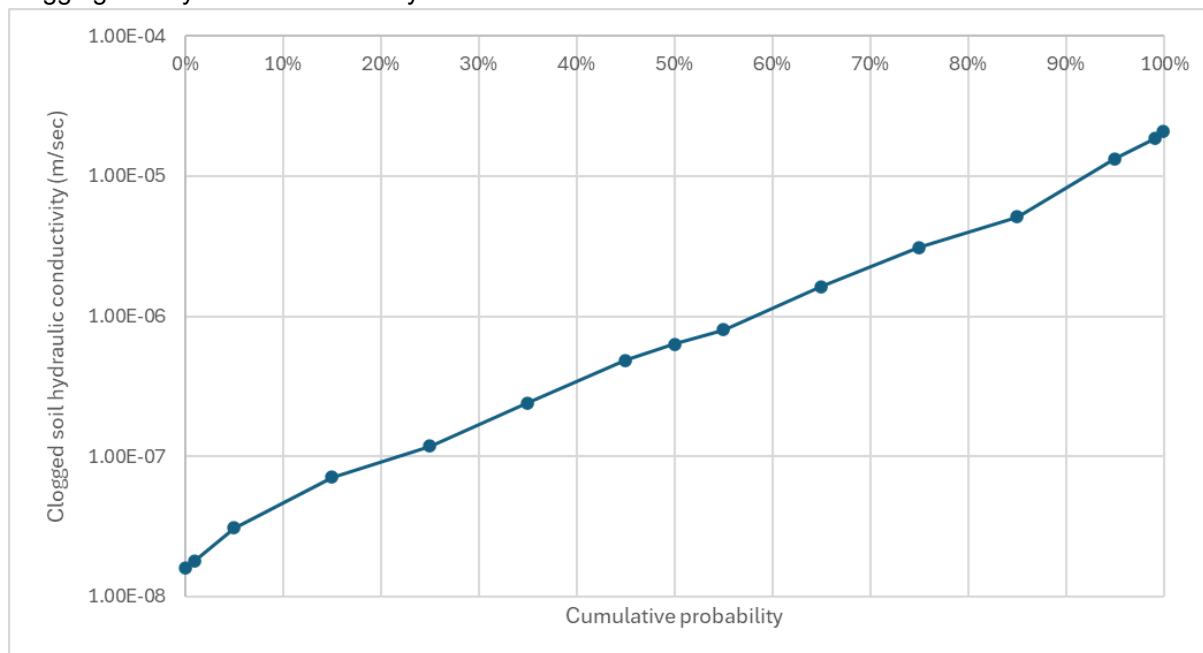
Figure E-4 Range of transmissivity and clogging for the soakholes on Frankton
