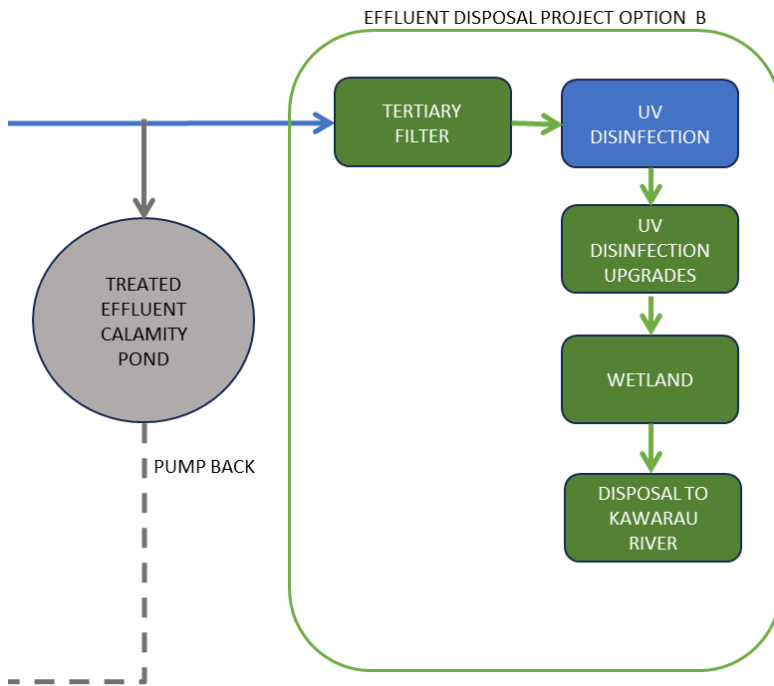
Figure 26 Shotover WWTP process including the Option B disposal
