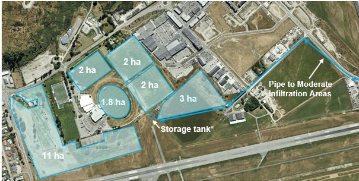
Figure 22 Indicative pipe route and estimated potential irrigation area in the golf course and sportfields
