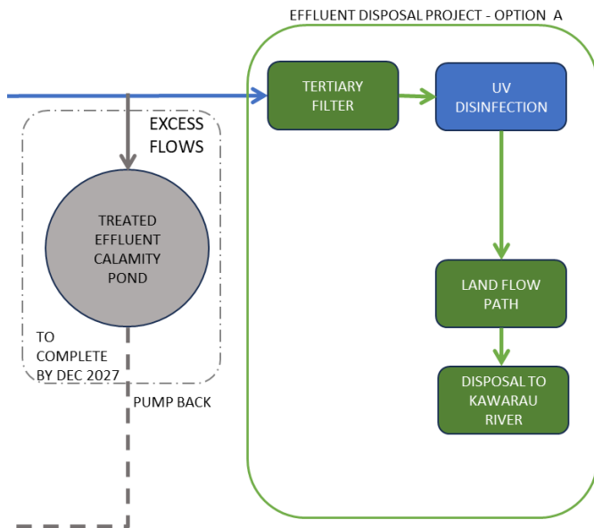
Figure 24 Process diagram for Option A
