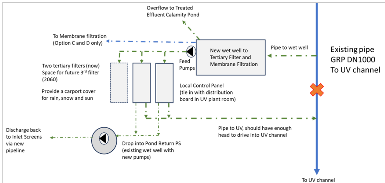
Figure 12 Tertiary filter concept arrangement
