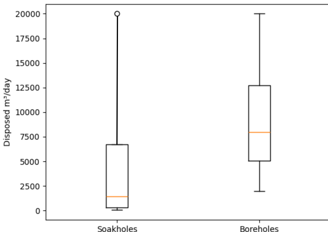
Figure E-7 Estimated discharge rates for Soakholes and Boreholes and the probability of achieving this.
