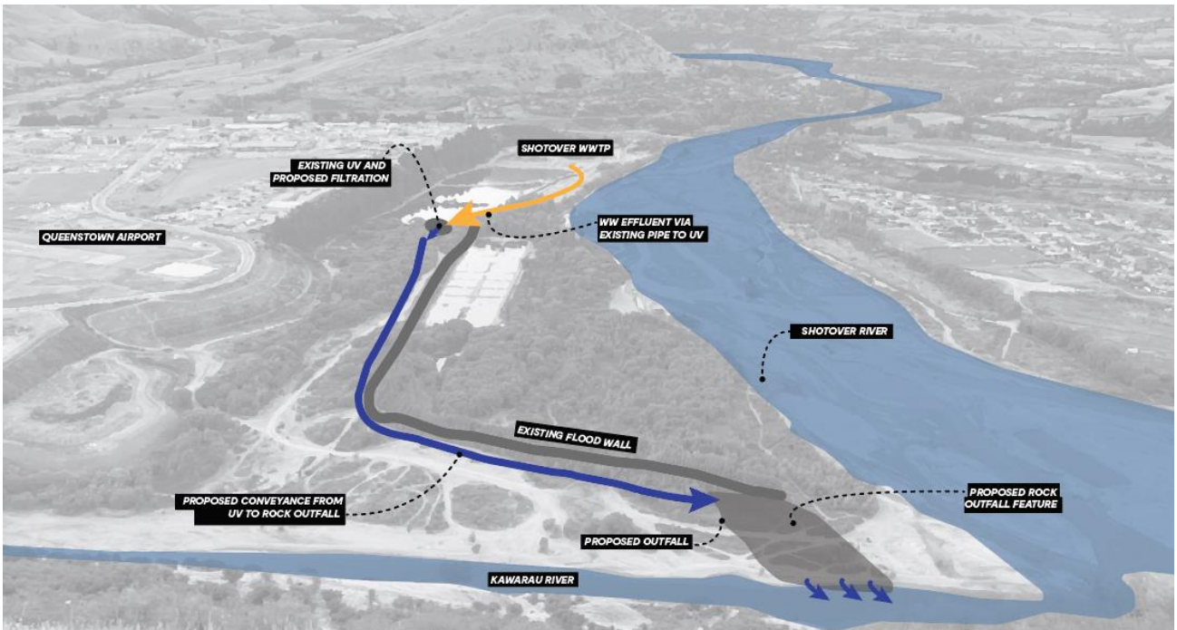
Figure i Option A indicative sketch
