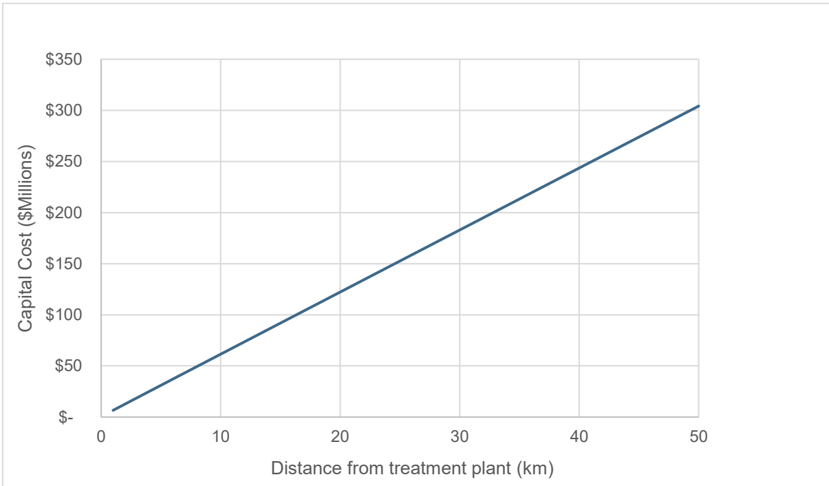
Figure 3 Rough order capital cost of conveyance compared to distance from treatment plant
