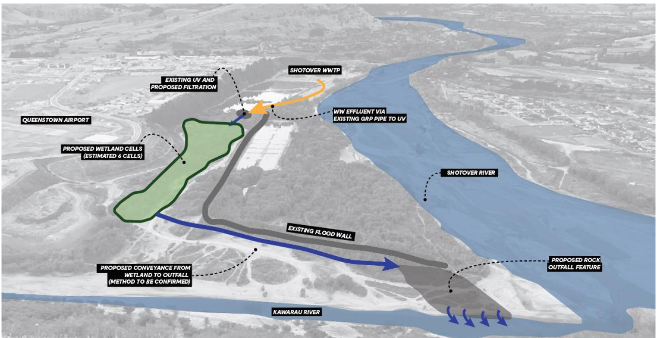
Figure ii Option B indicative sketch
