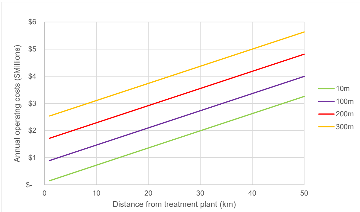
Figure 4 Annual operating costs for a range of distances and elevations
