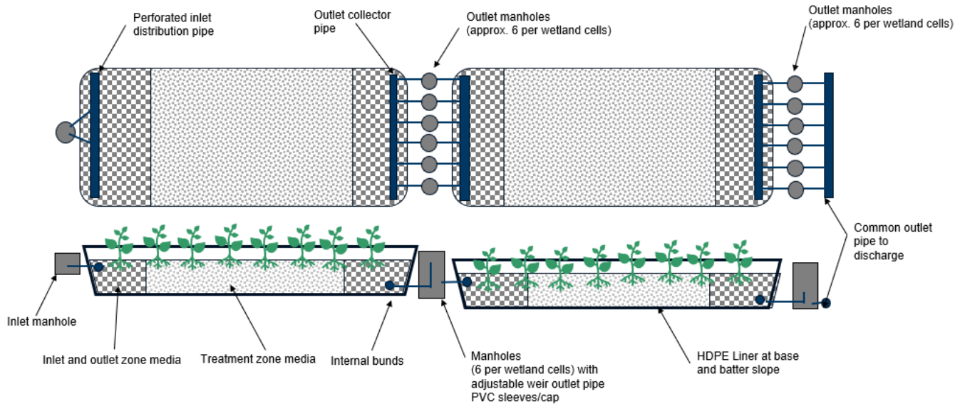
Figure 17 Subsurface wetland conceptual schematic
