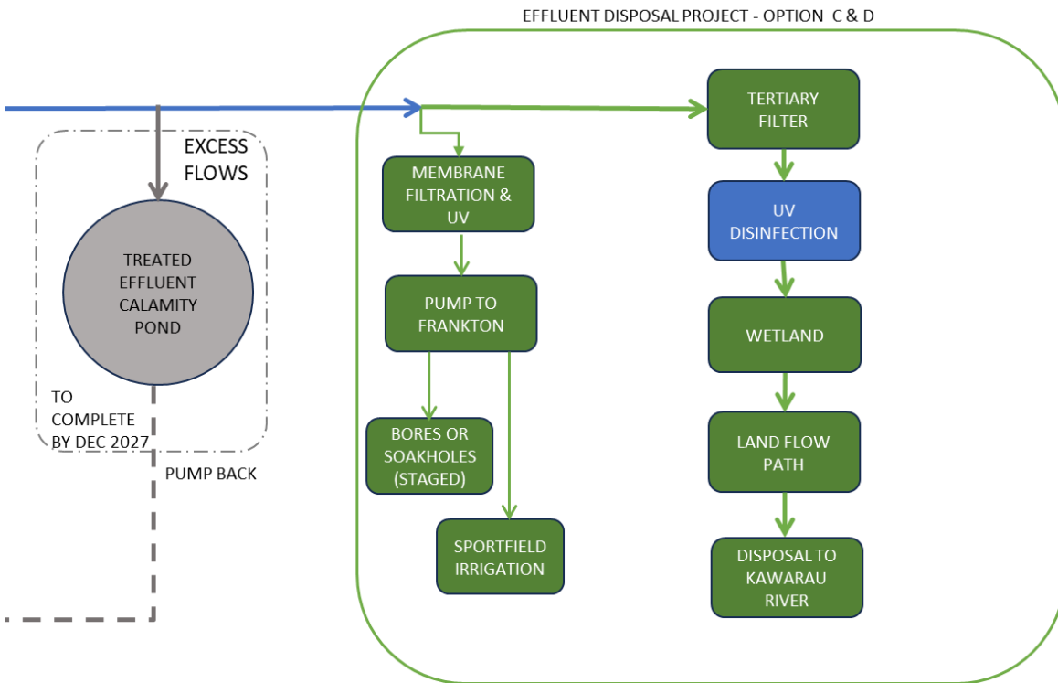
Figure 28 Shotover WWTP process including the Option C disposal.
