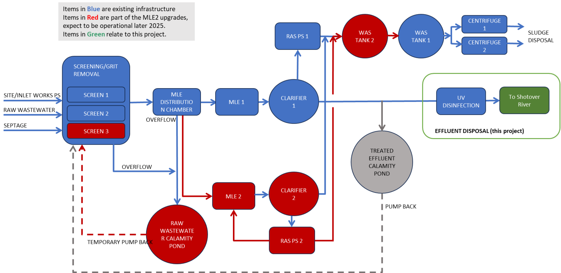
Figure 2 Shotover WWTP existing set up, Stage 3 upgrade, and project extent schematic
