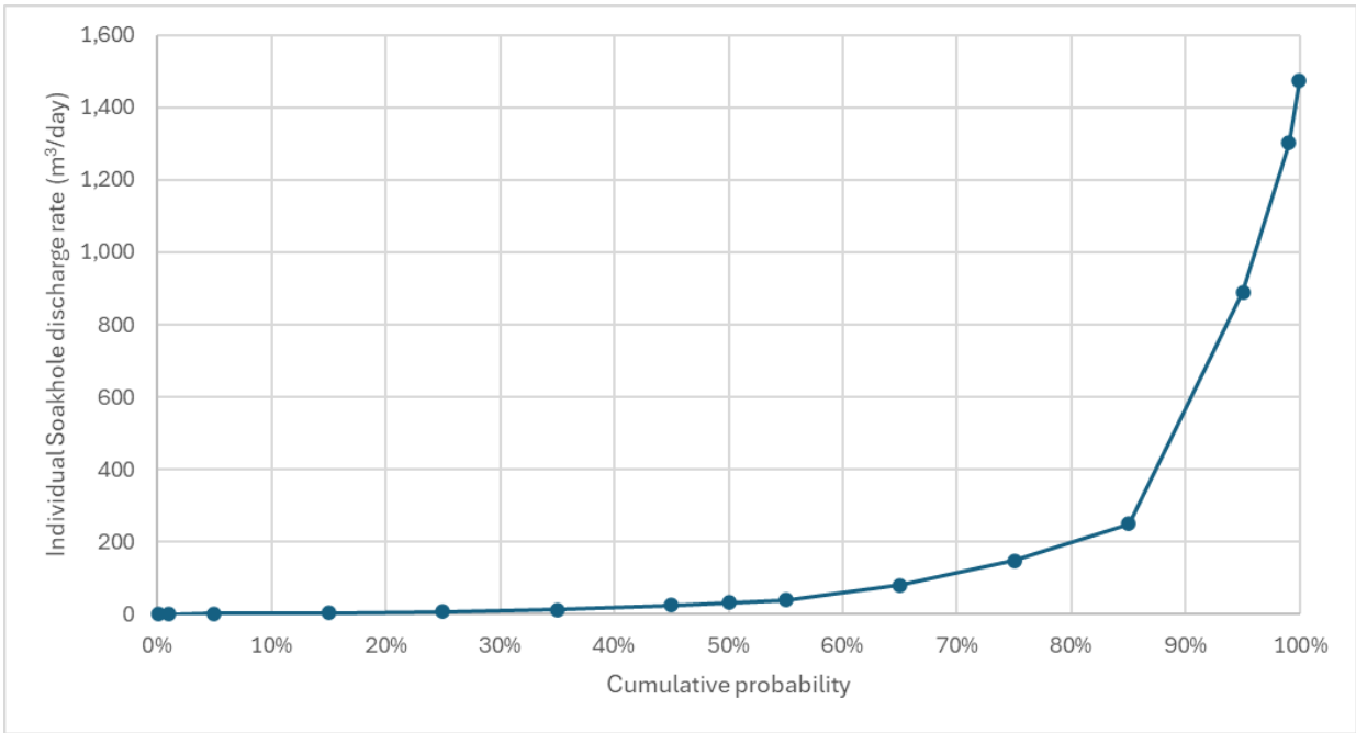
Figure E-5 Individual soakhole discharge rate
