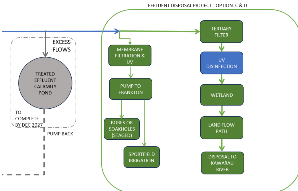
Figure 30 Shotover WWTP process including Option D disposal
