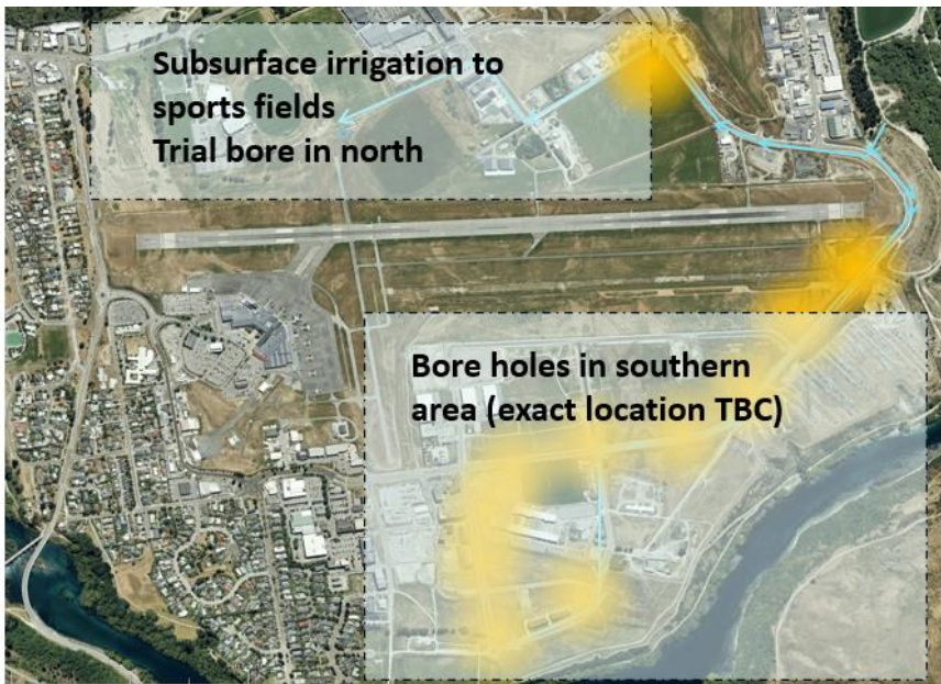
Figure 29 Option C Bore injection indicative location
