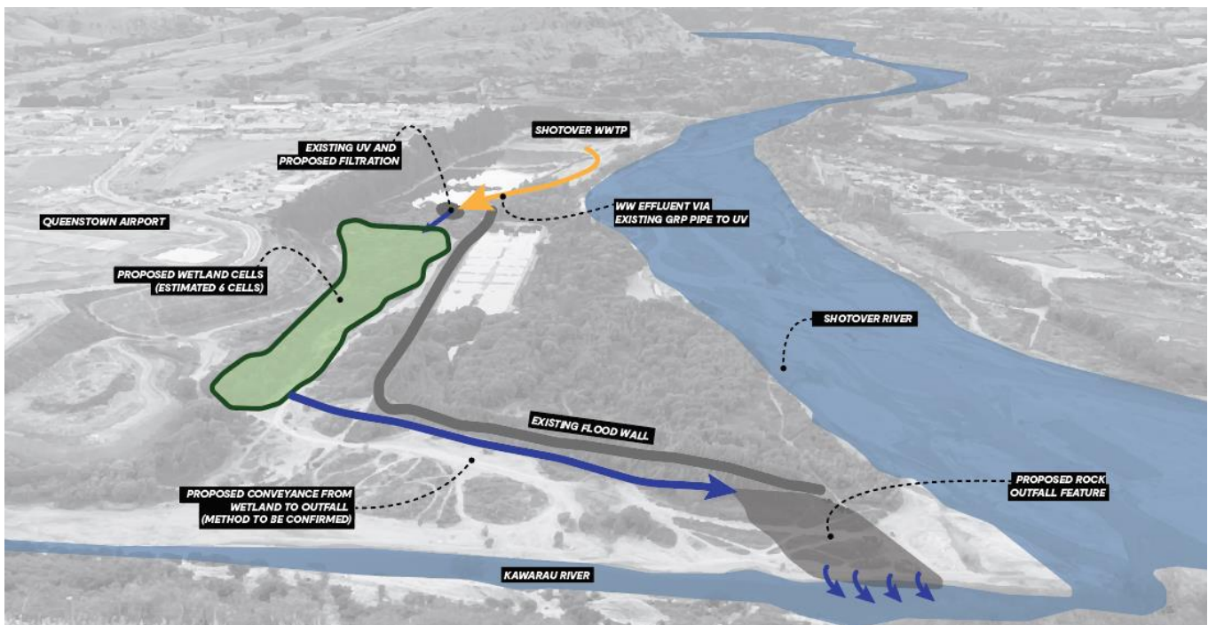
Figure 27 Option B - Wetland schematic illustration
