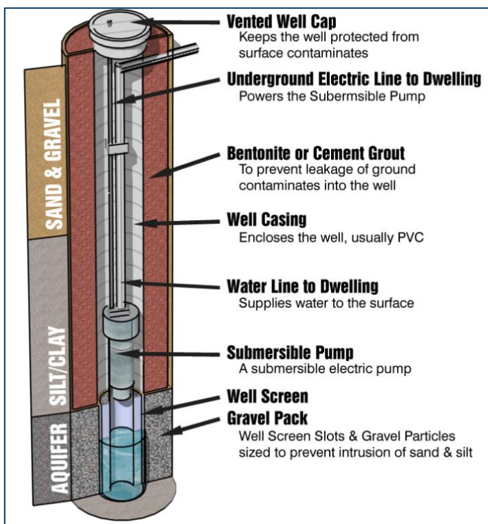
Figure 21 Typical bore construction (Harvard University, 2016), details to be confirmed in preliminary design phase
