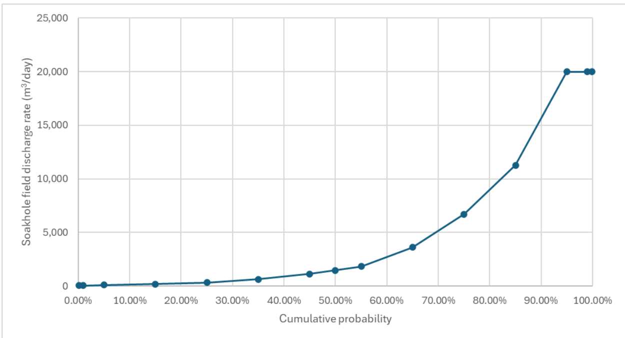
Figure E-6 Combined soakhole discharge rate (50 soakholes)
