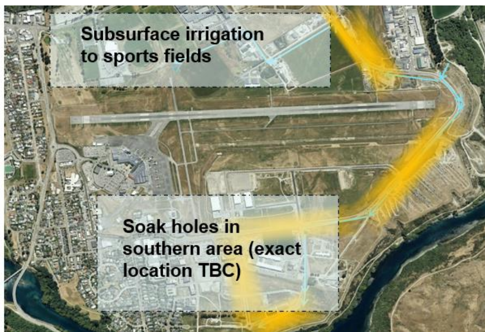
Figure 31 Option D Soakhole indicative location plan
