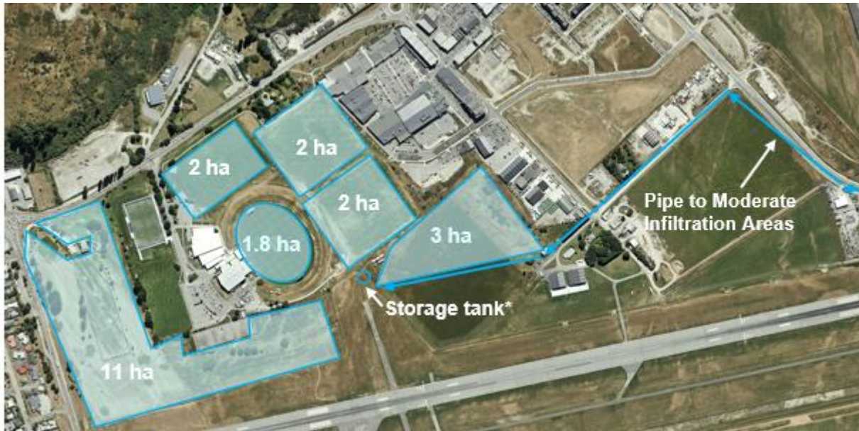
Figure 6 Estimated irrigation area in the golf course and sport fields
