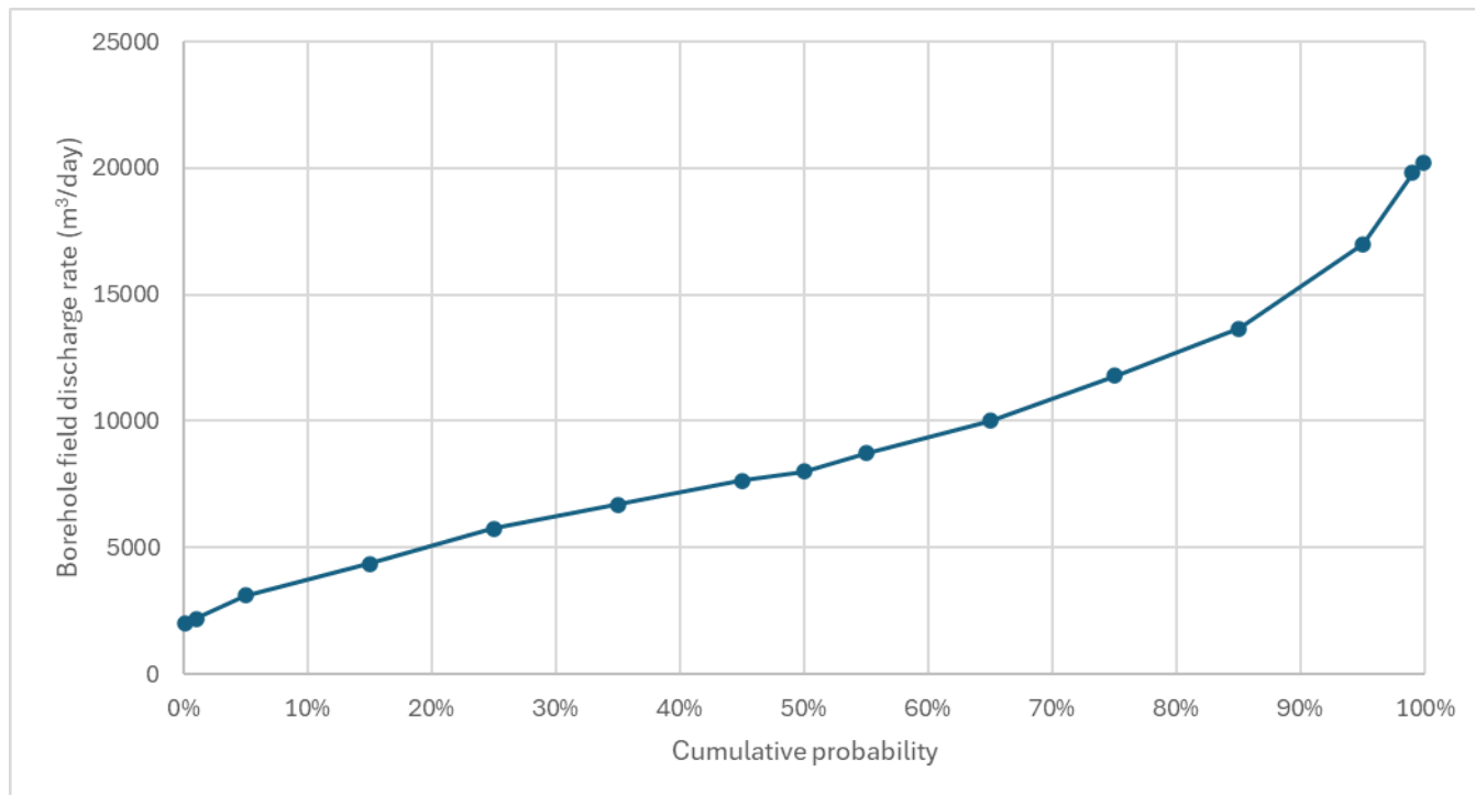
Figure E-3 Combined borehole discharge rate (total of 10 bores)
