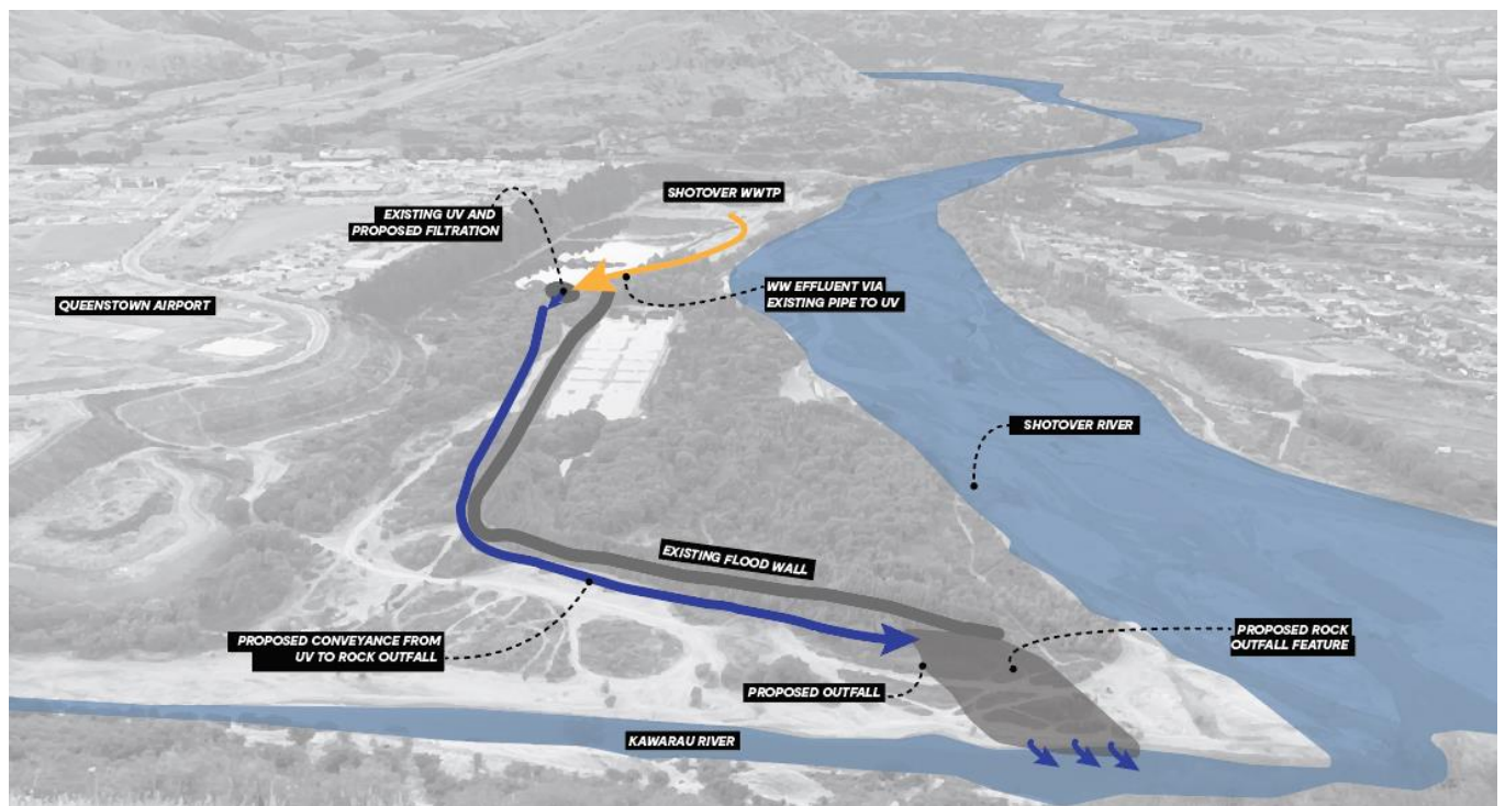
Figure 25 Option A Rock outfall schematic illustration
