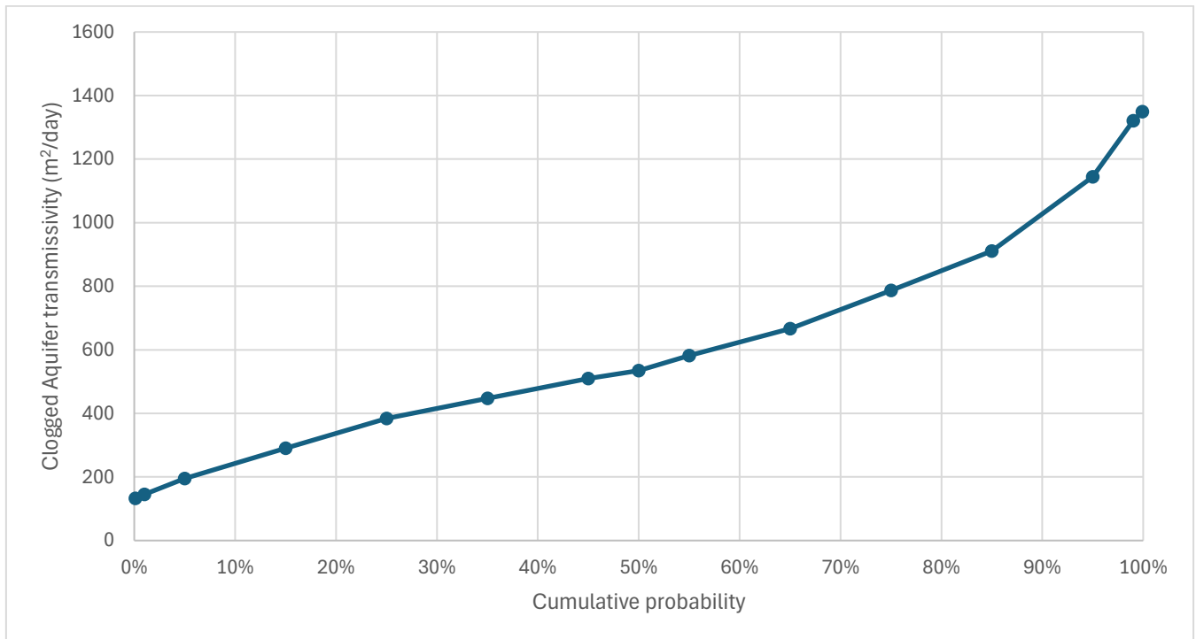
Figure E-1 Range of transmissivity and clogging for the boreholes on Frankton.
