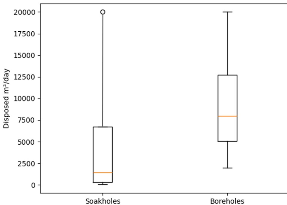
Figure 7 Estimated discharge rates for soak holes and boreholes and the probability of achieving this
