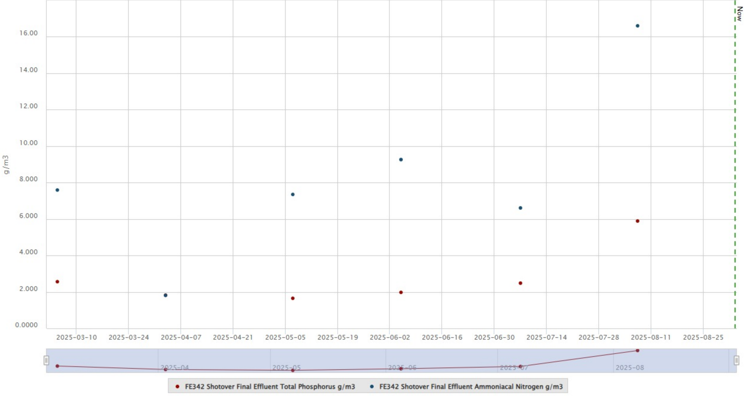
FE342 - Condition 12 - Total Phosphorus and Ammoniacal Nitrogen g/m3
