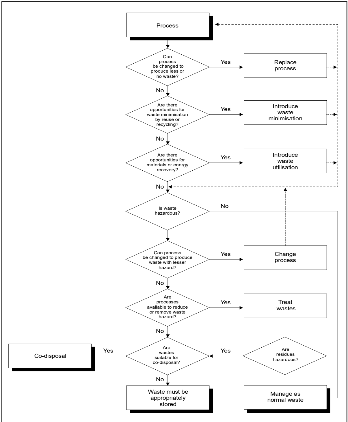
Figure 3: Evaluation of a waste producing process and the management of potentially hazardous waste (Adapted from Ministry for the Environment (1993) New Zealand Waste Hazardous Substances Handbook, Figure 3.1 & 3.2)
